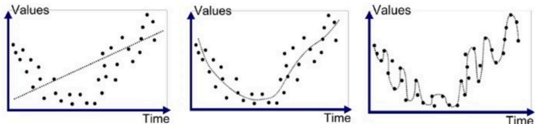
Underfitted
